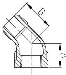
Street Elbow, 45°
