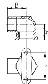
Drop Ear 90° Elbow
