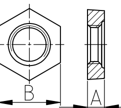
Locknut
