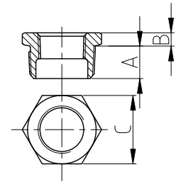
Outside Hex Bushing
