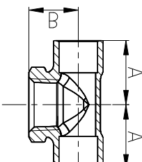
Adapter Tee
