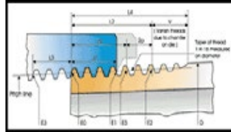
Taper thread
