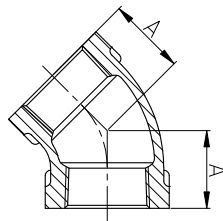
Street Elbow, 45°
