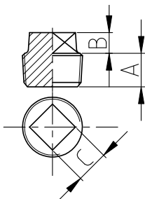
Solid Plug
