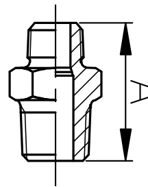
Hexagon Nipple
