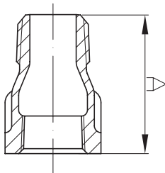
Cored Plug
