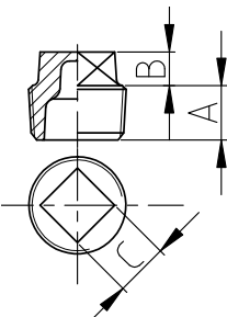
Solid Plug
